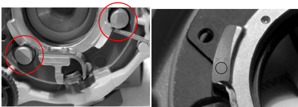
Figure 10a+b - Detail view (from below) of the upper tribrach plate showing the instrument released (a); Detail view of a clamping flange (b)
