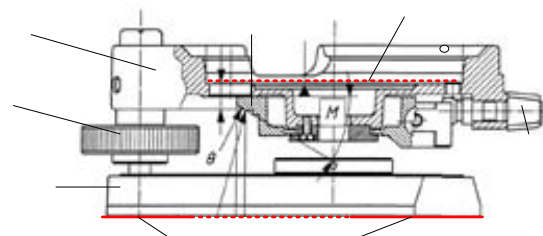
Figure 1 - Cross section of a Leica GDF121 tribrach
