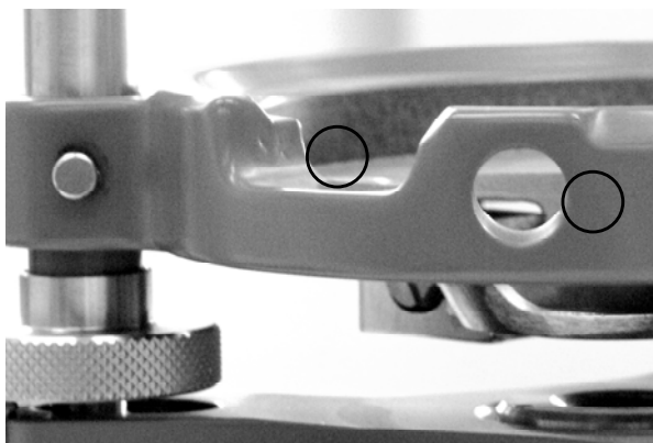
Figure 6 - Detail view of WILD GDF6 tribrach
